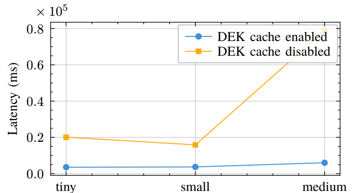
Figure 3. DEK cache impact on cold GET latency
